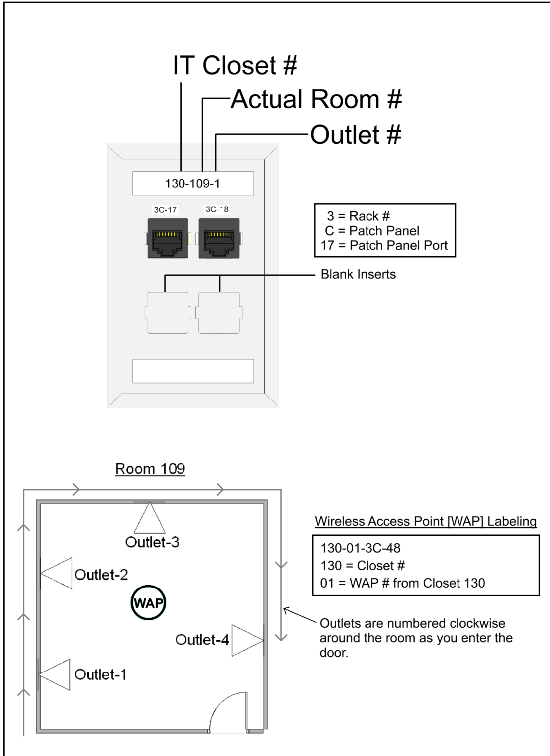
Figure 12.3 – Labeling Legend Detail
