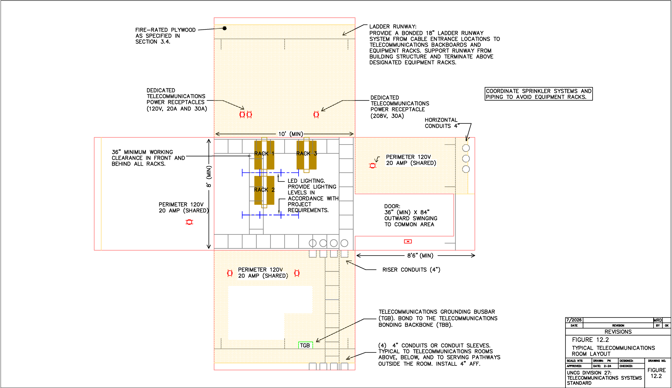
Figure 12.2 – Typical Telecommunications Room Layout
