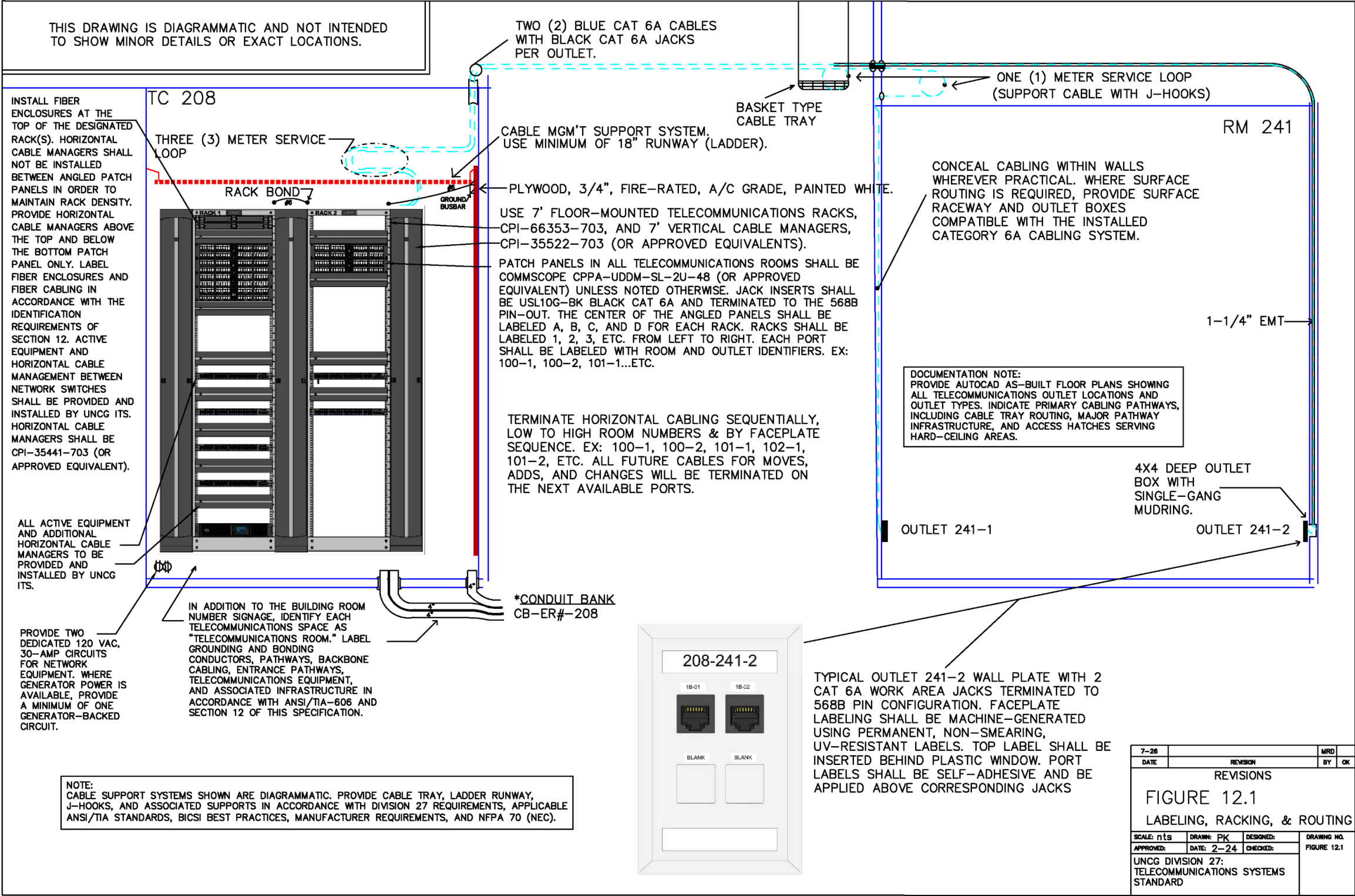
Figure 12.1 – Labeling, Racking, & Routing
